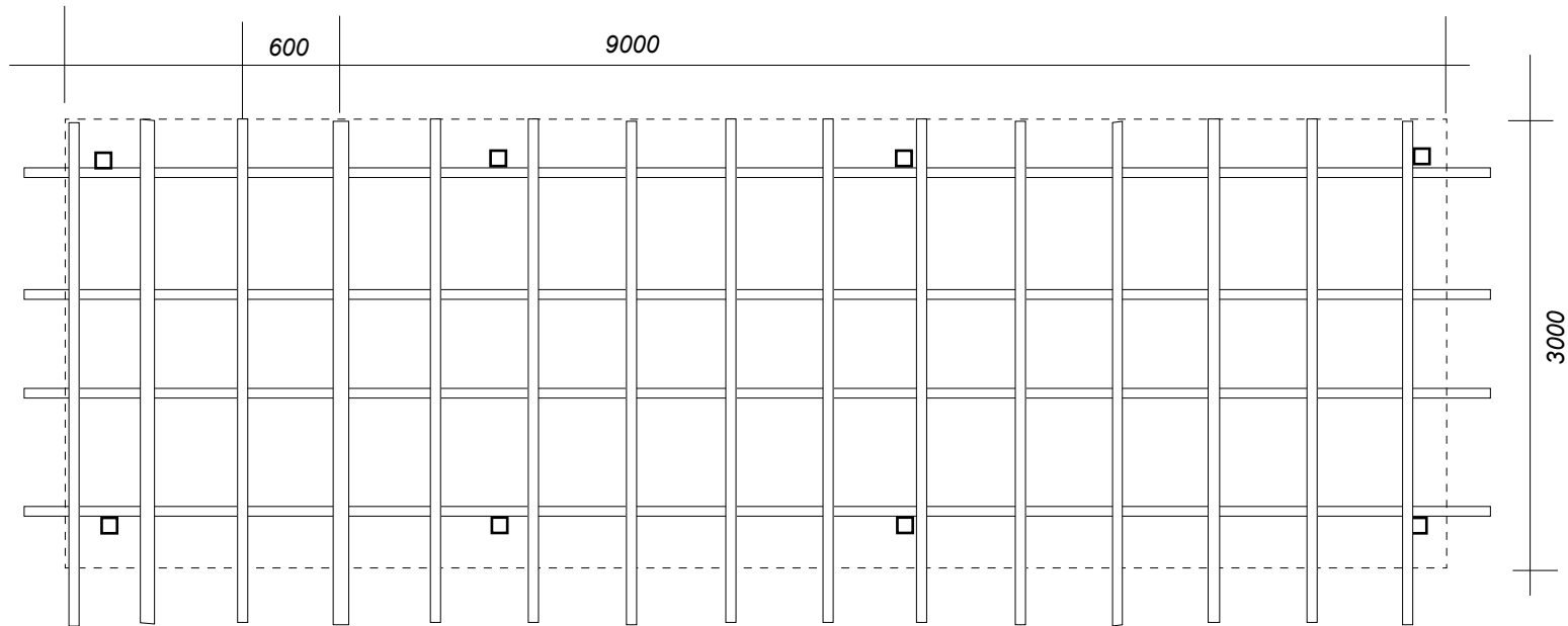
Roof frame
